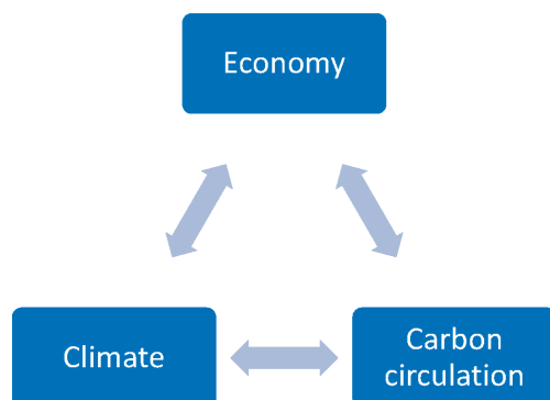
Figure 23.2: Integrated Assessment Models, IAMs, consist of three building blocks: an economy, a representation of the carbon cycle, and a climate module.
